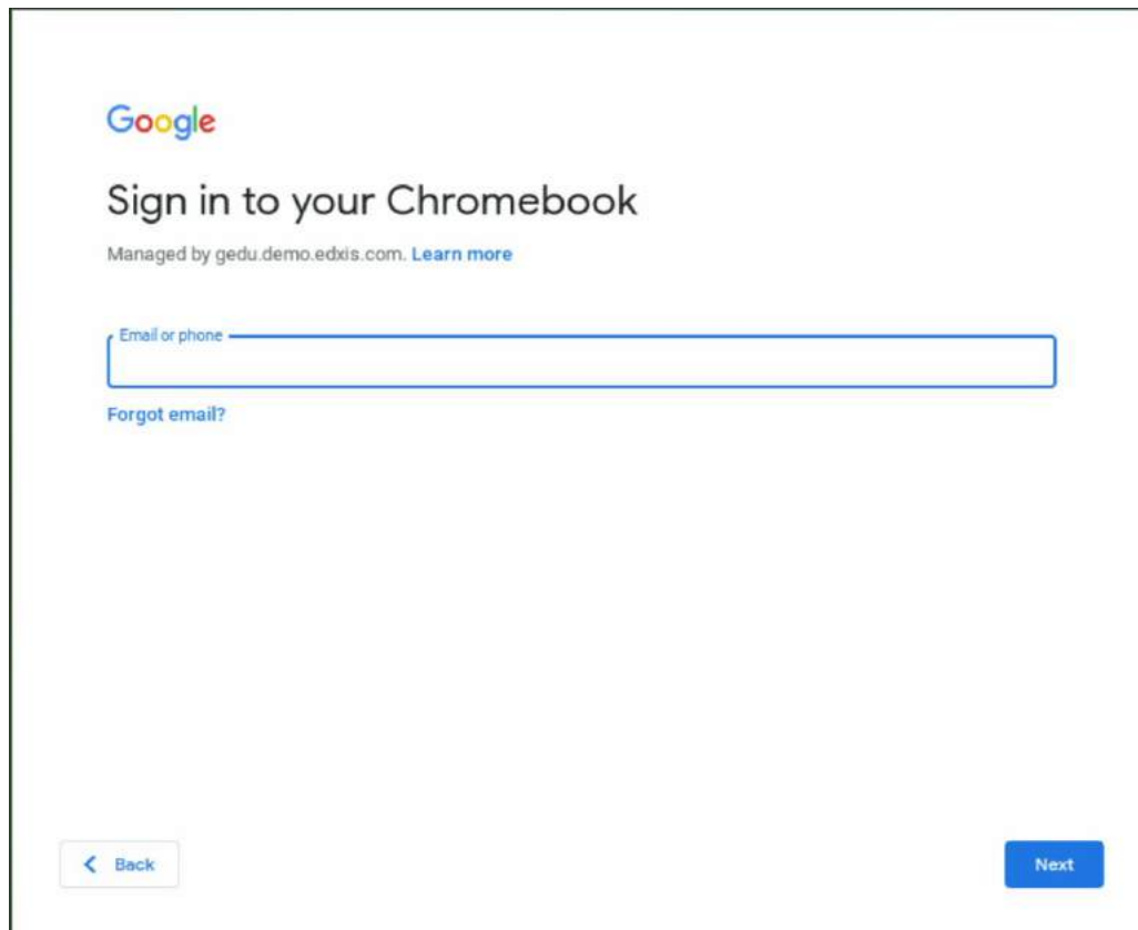
Figure 2.1: Login screen
